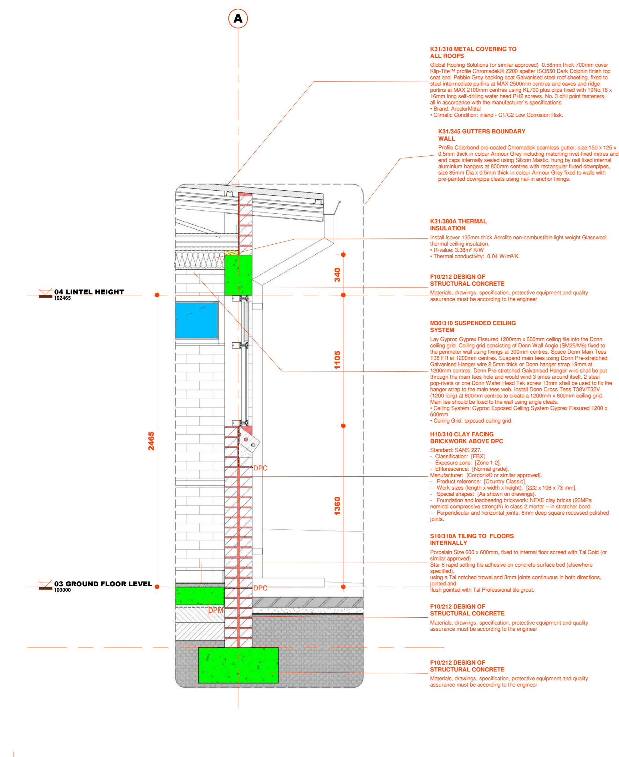
SECTION G-G - Callout 1 1:20
