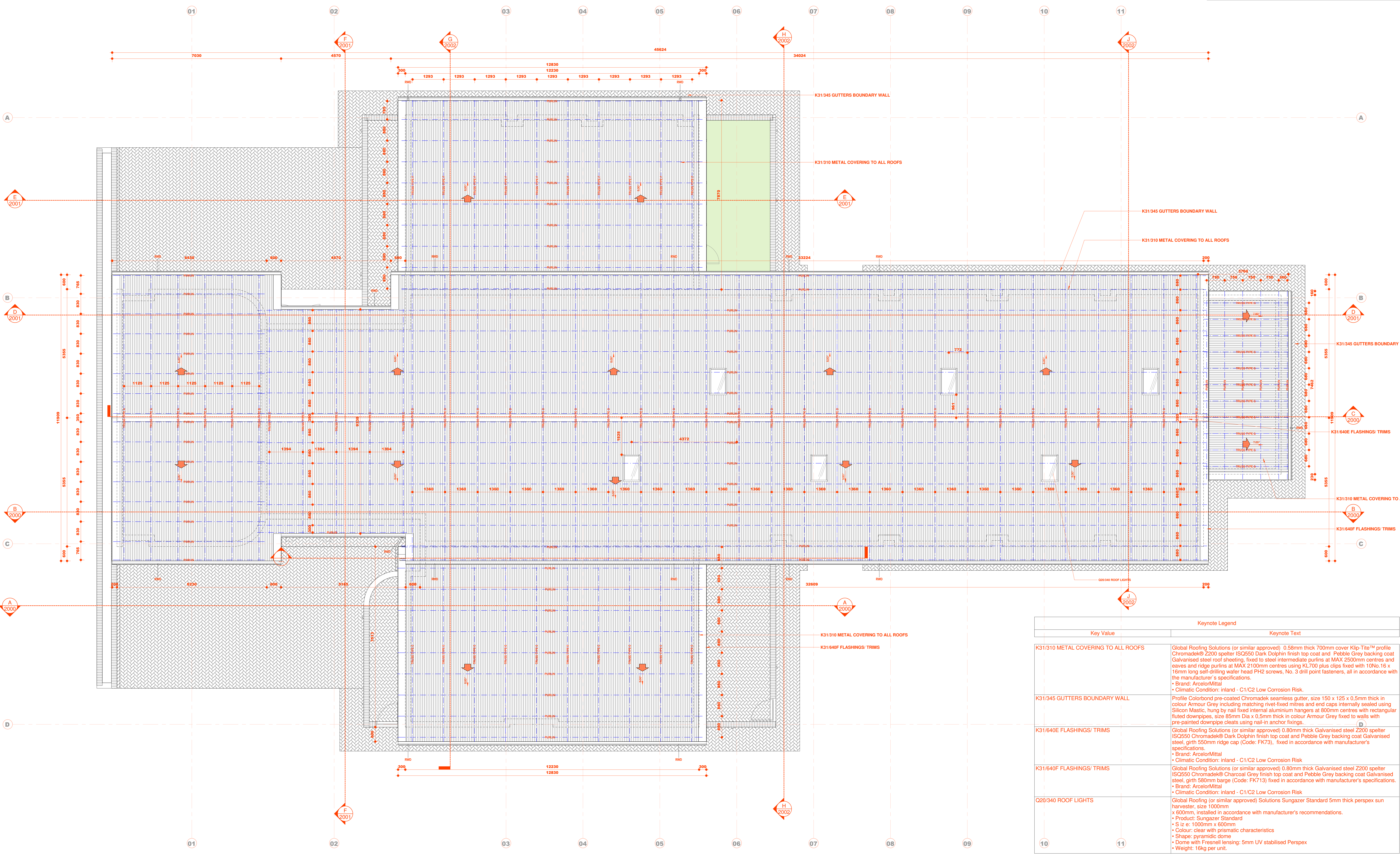
1500 - ROOF PLAN 1:50
