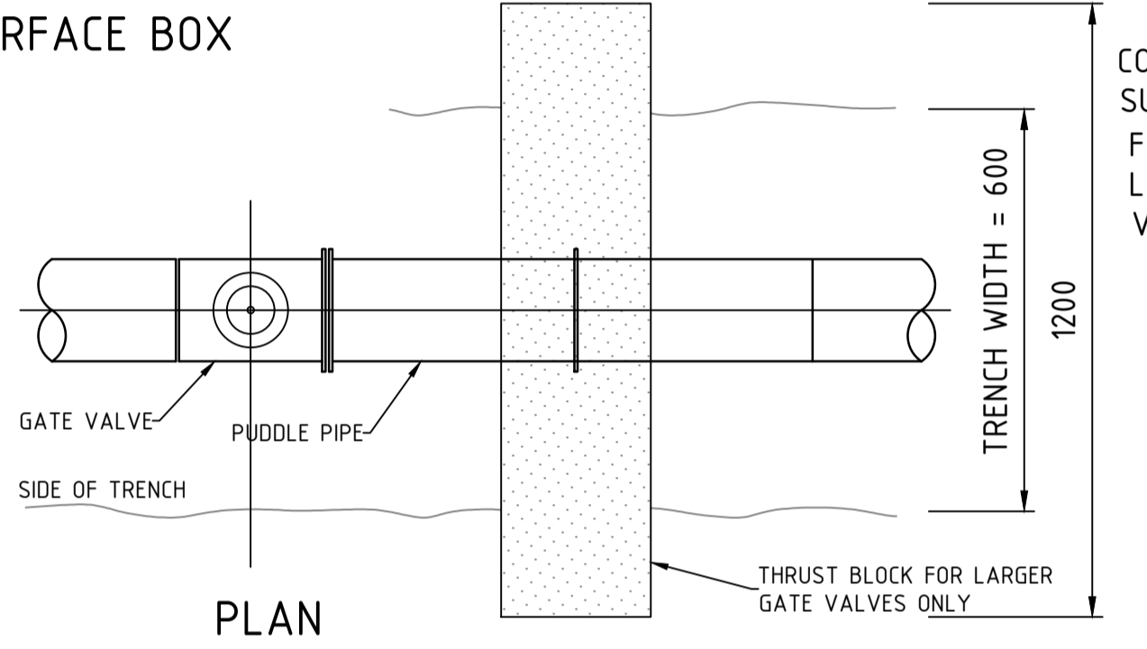
GATE VALVE TYPE II SCALE: NTS
