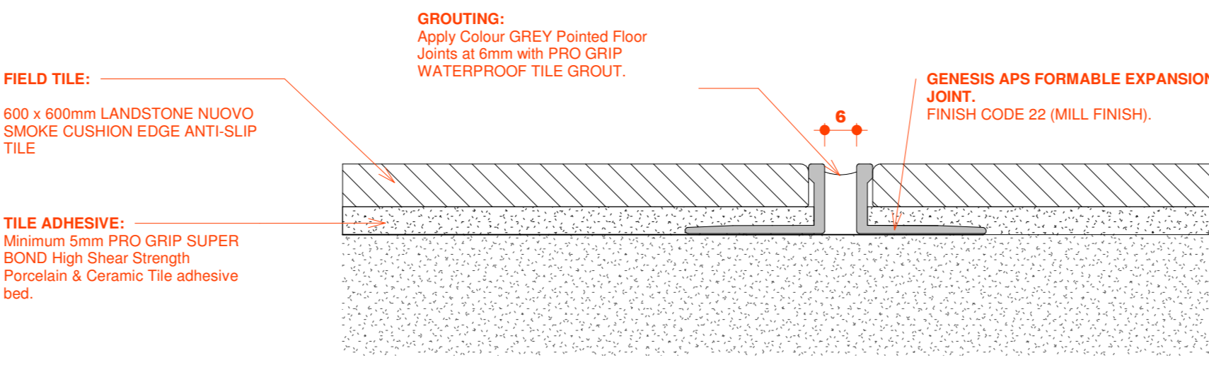
TYPICAL TILE MOVEMENT JOINT 1:1
