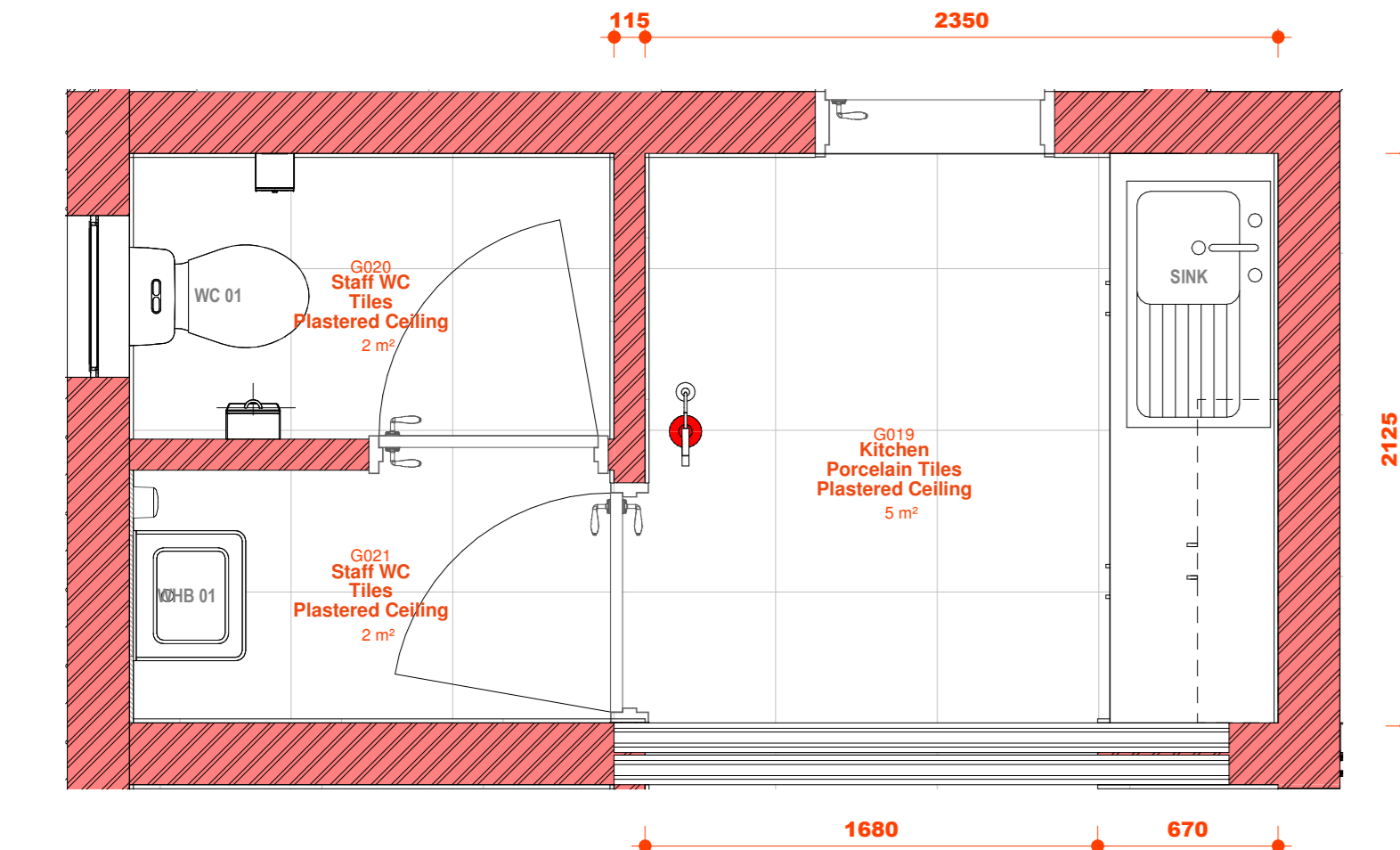
03 GROUND FLOOR LEVEL - G019 1:25
