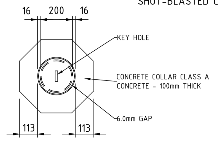
PLAN TO SURFACE BOX
