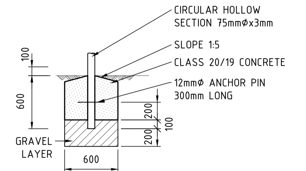
FOUNDATION DETAIL SCALE 1:25
