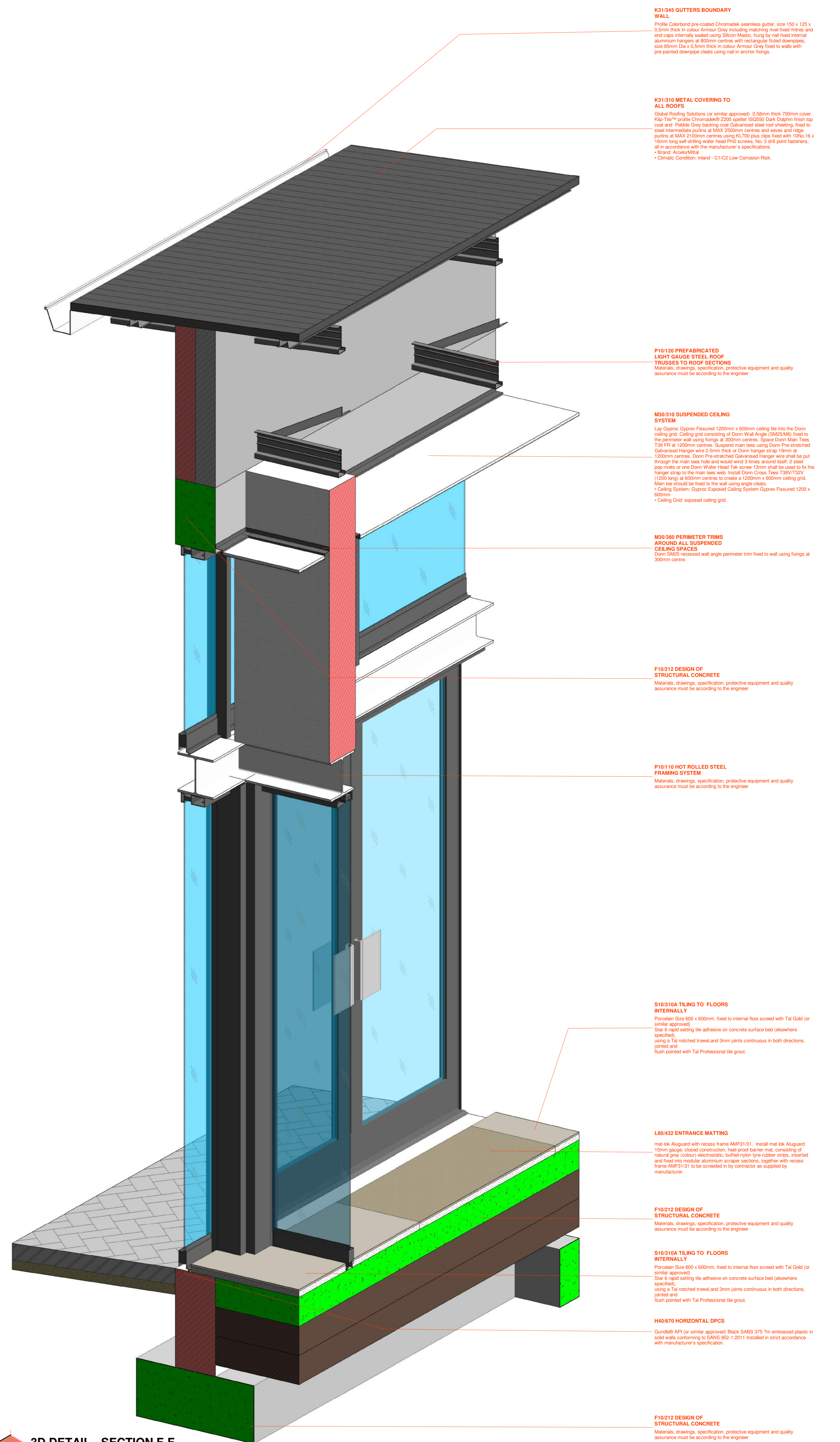
3D DETAIL - SECTION F-F 1:3
