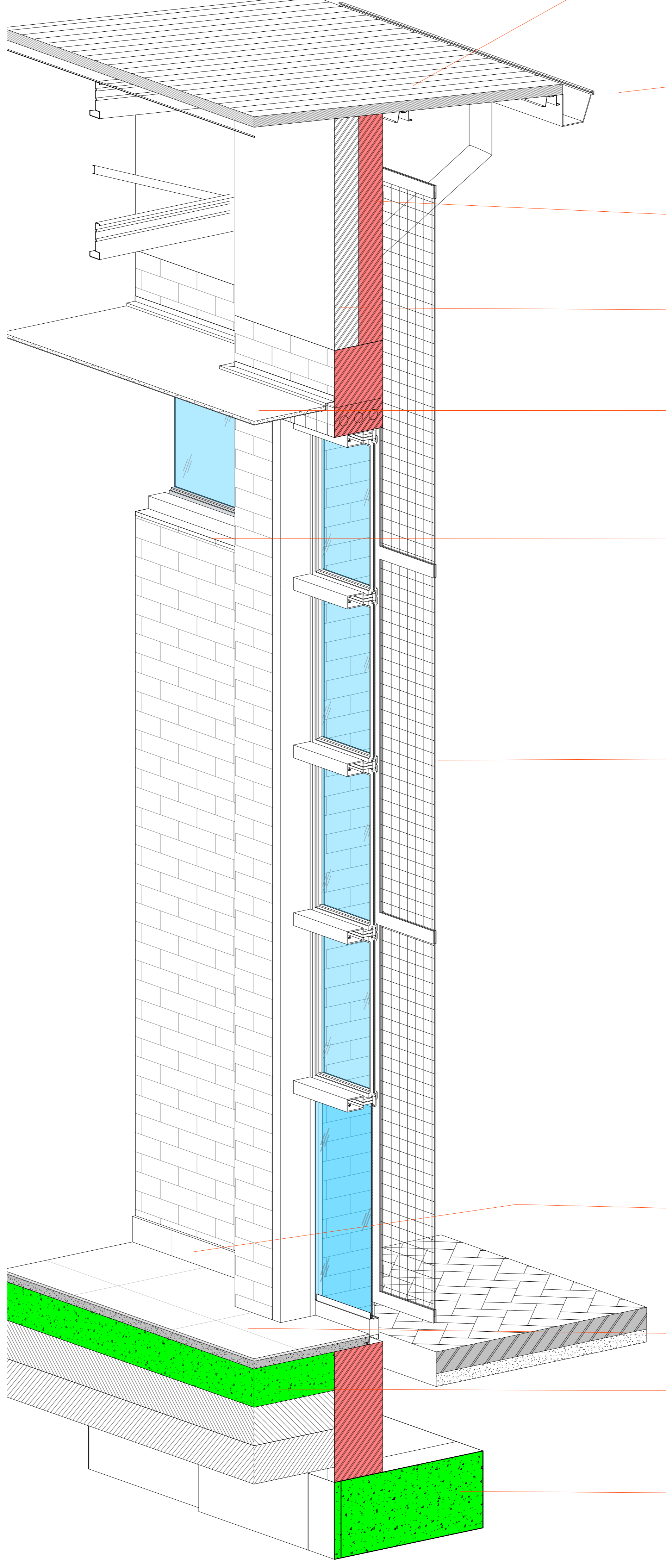
3D DETAIL 1:20
