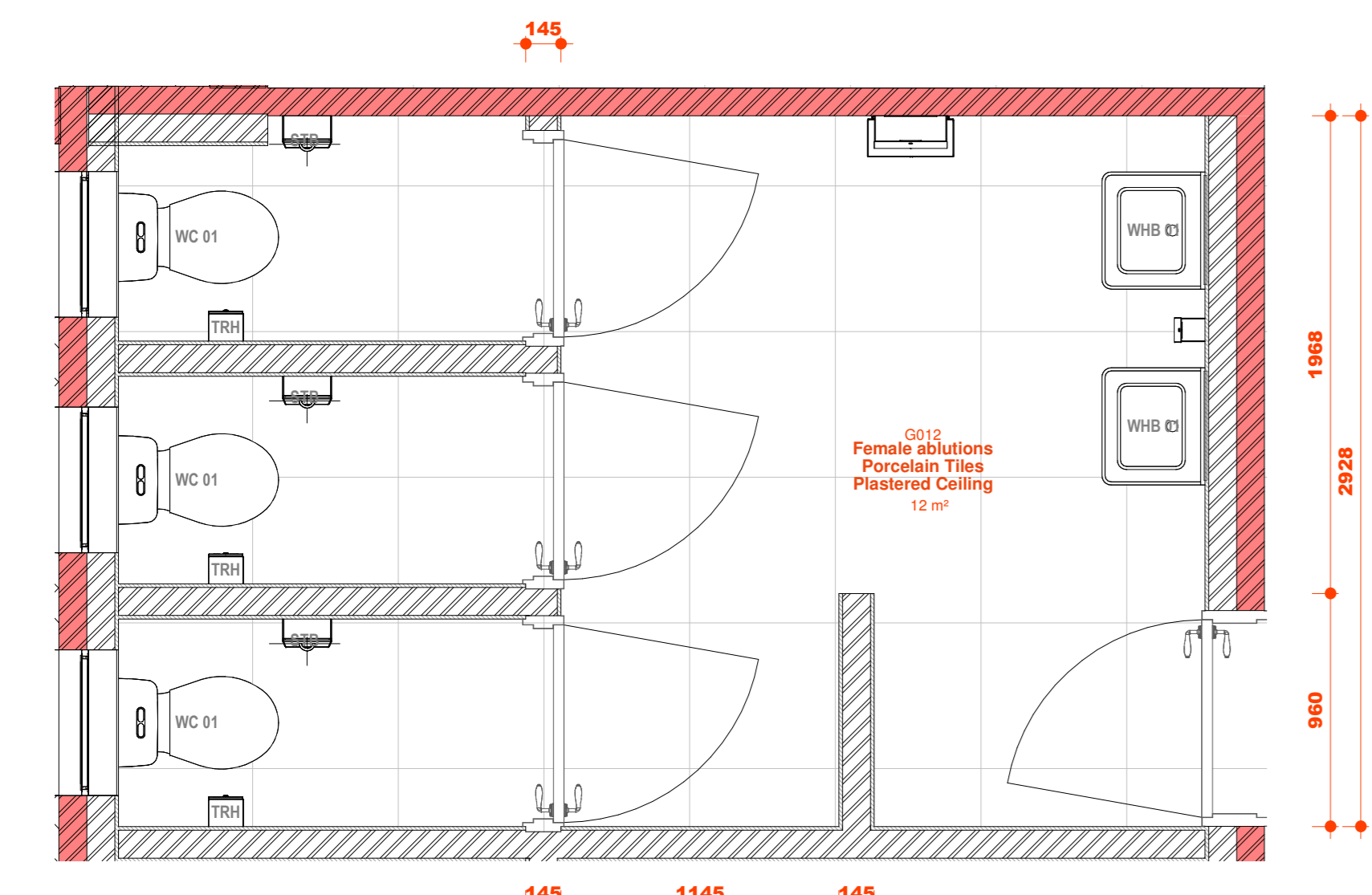
03 GROUND FLOOR LEVEL - G012 1:25
