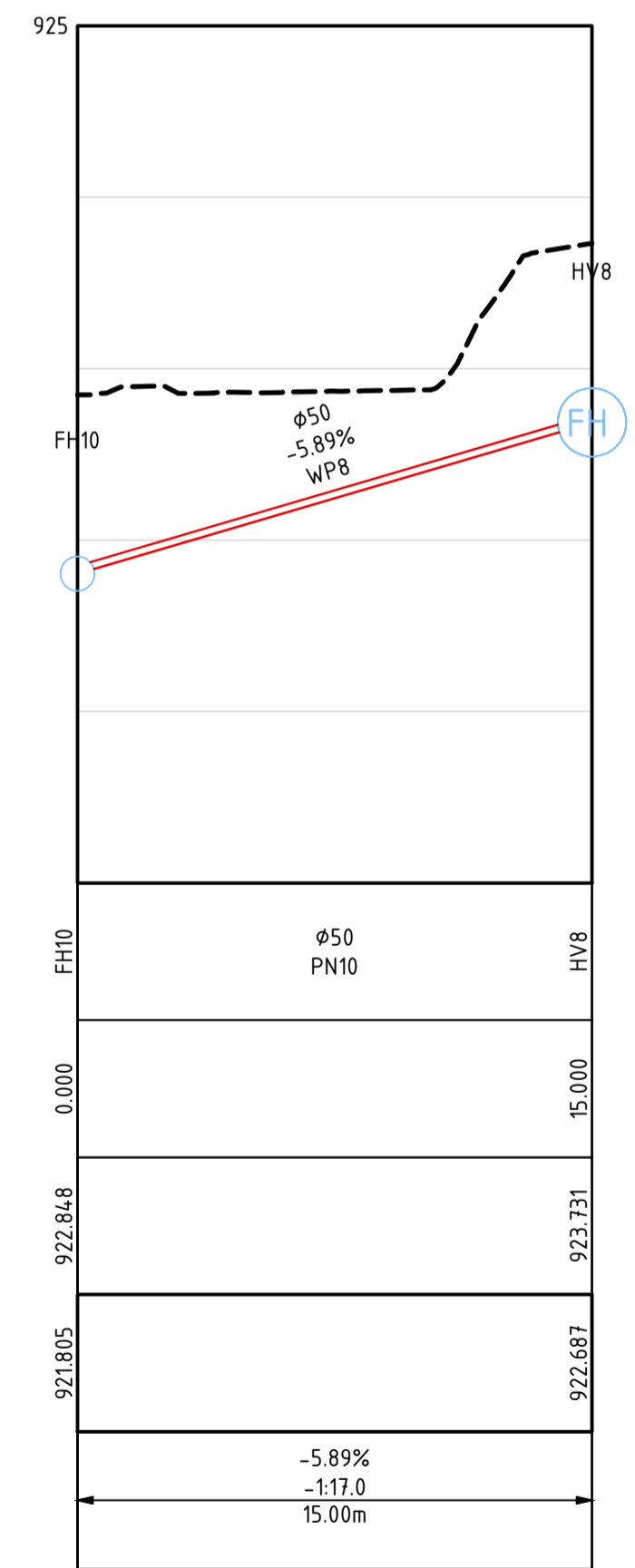
LONGSECTION FH10 - HV8 FROM 0.000 TO 15.000
