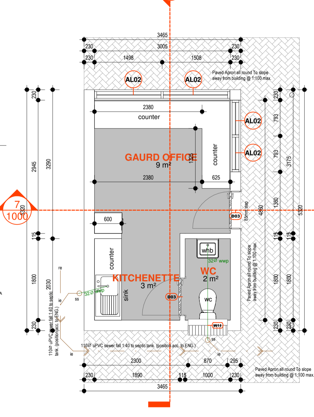
1 100 GROUND FLOOR LEVEL 1:50
