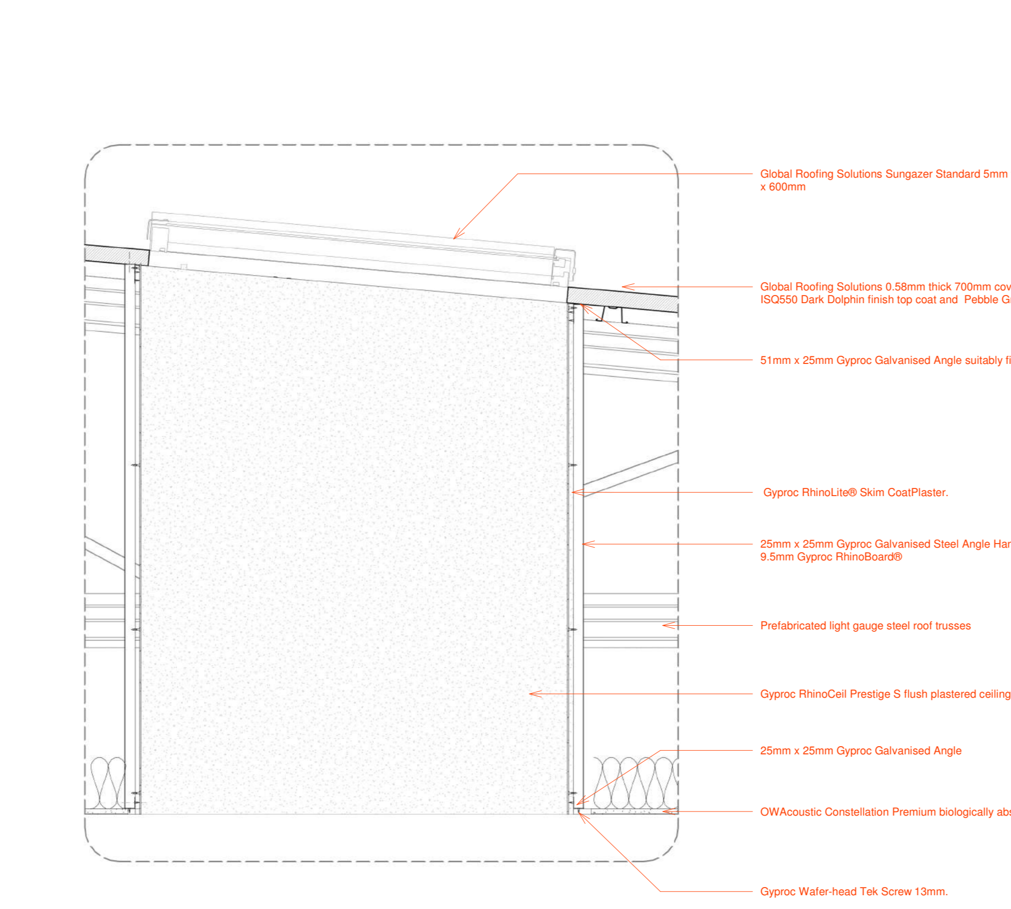
LIGHTWELL BULKHEAD DETAIL 1:10
