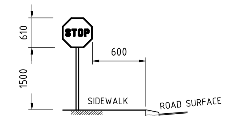
MOUNTING OF ROAD SIGN SCALE 1:25
