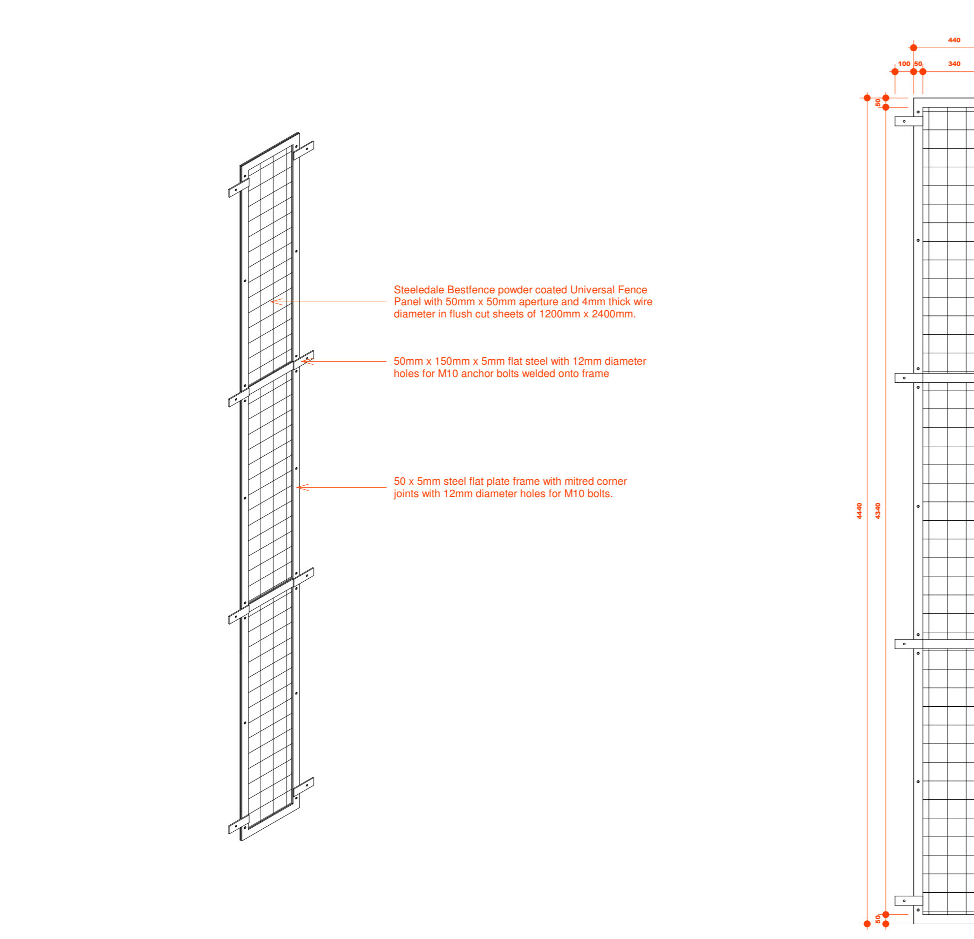
BURGLAR PROOFING 1:20
