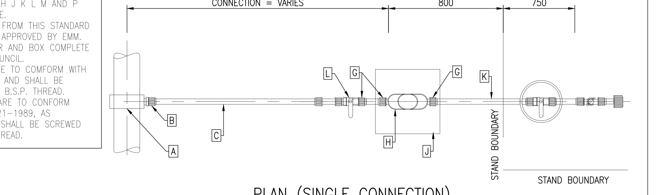
STANDARD HOUSE CONNECTION DETAIL SCALE NTS
