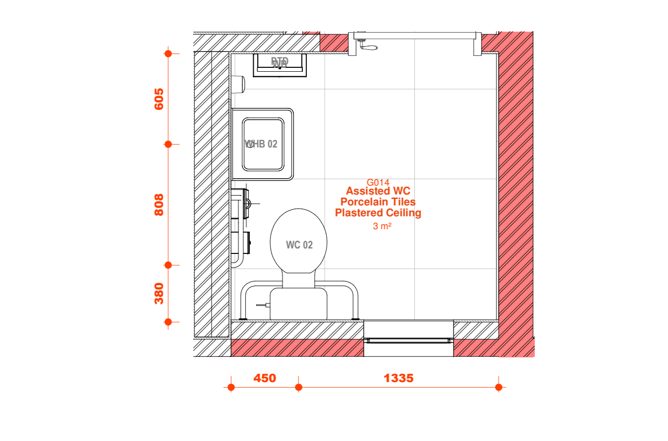
03 GROUND FLOOR LEVEL - G014 1:25
