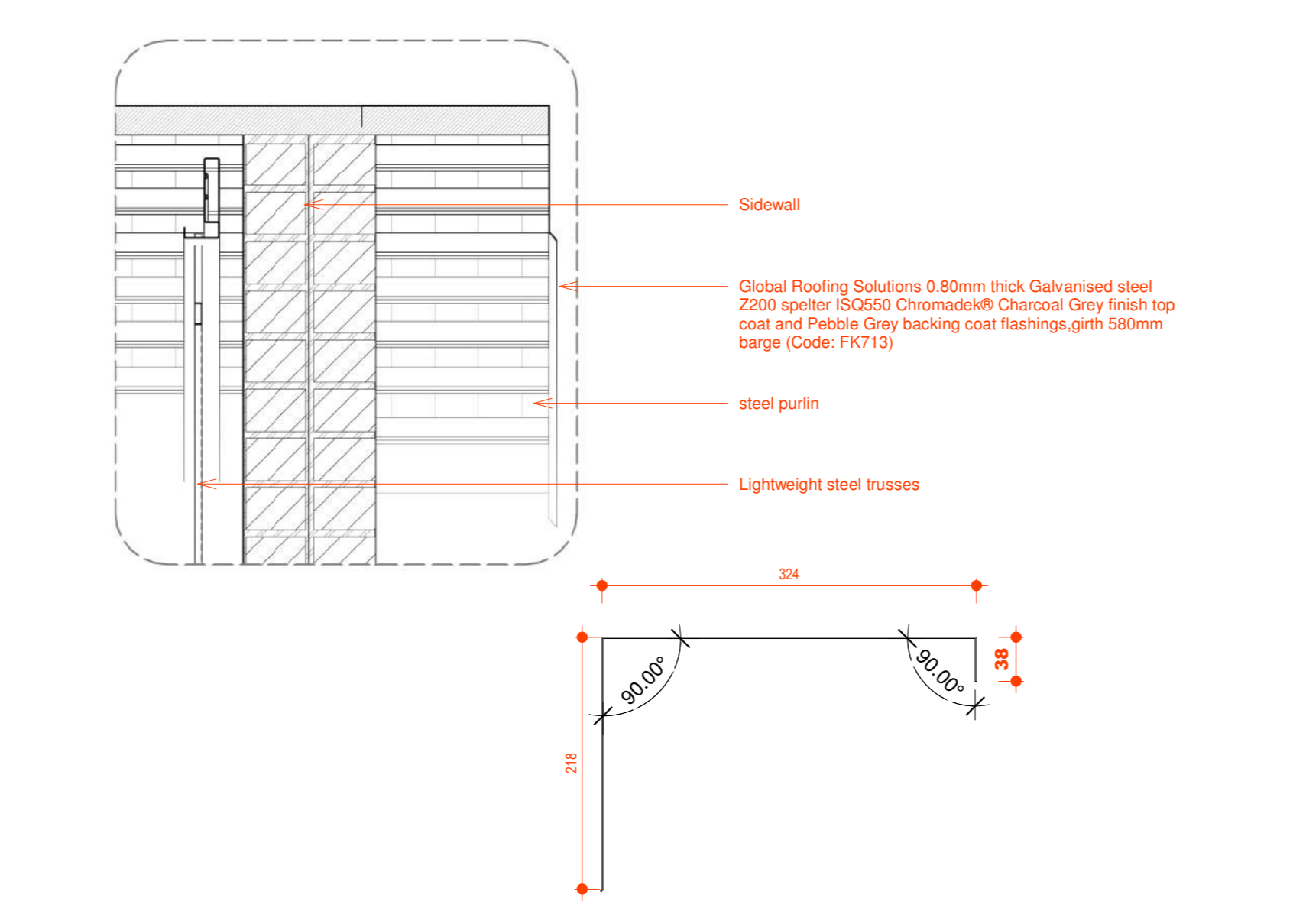
BARGE FLASHING DETAIL 1:10
