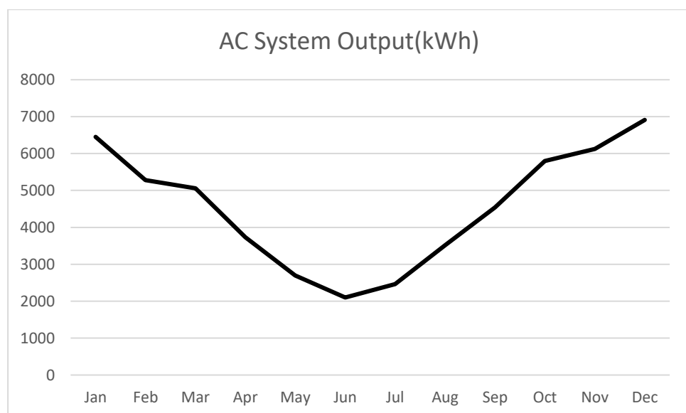
Figure 1. AC System Output for a 44.5 kWp Solar PV System in Vleifontein
