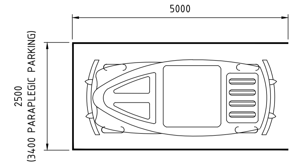
TYPICAL PARKING BAY LAYOUT SCALE 1:50
