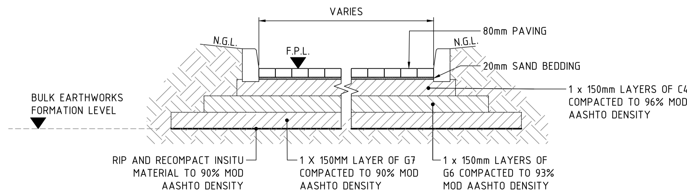
TYPICAL BULK EARTHWORKS SECTION FOR PARKING AREA AND ACCESS ROAD SCALE 1:20
