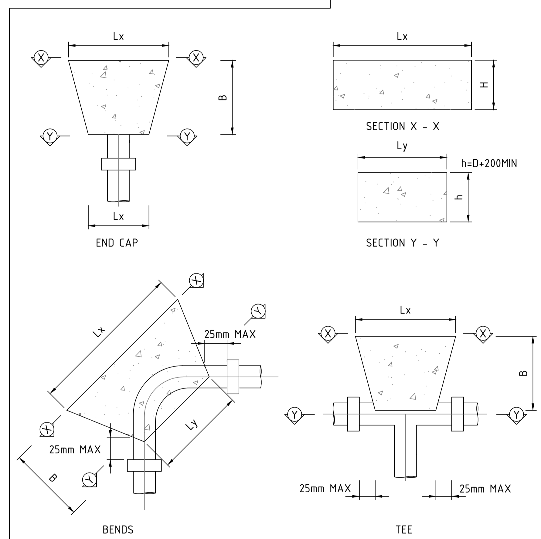
TYPICAL THRUSH BLOCK DETAILS SCALE 1:10
