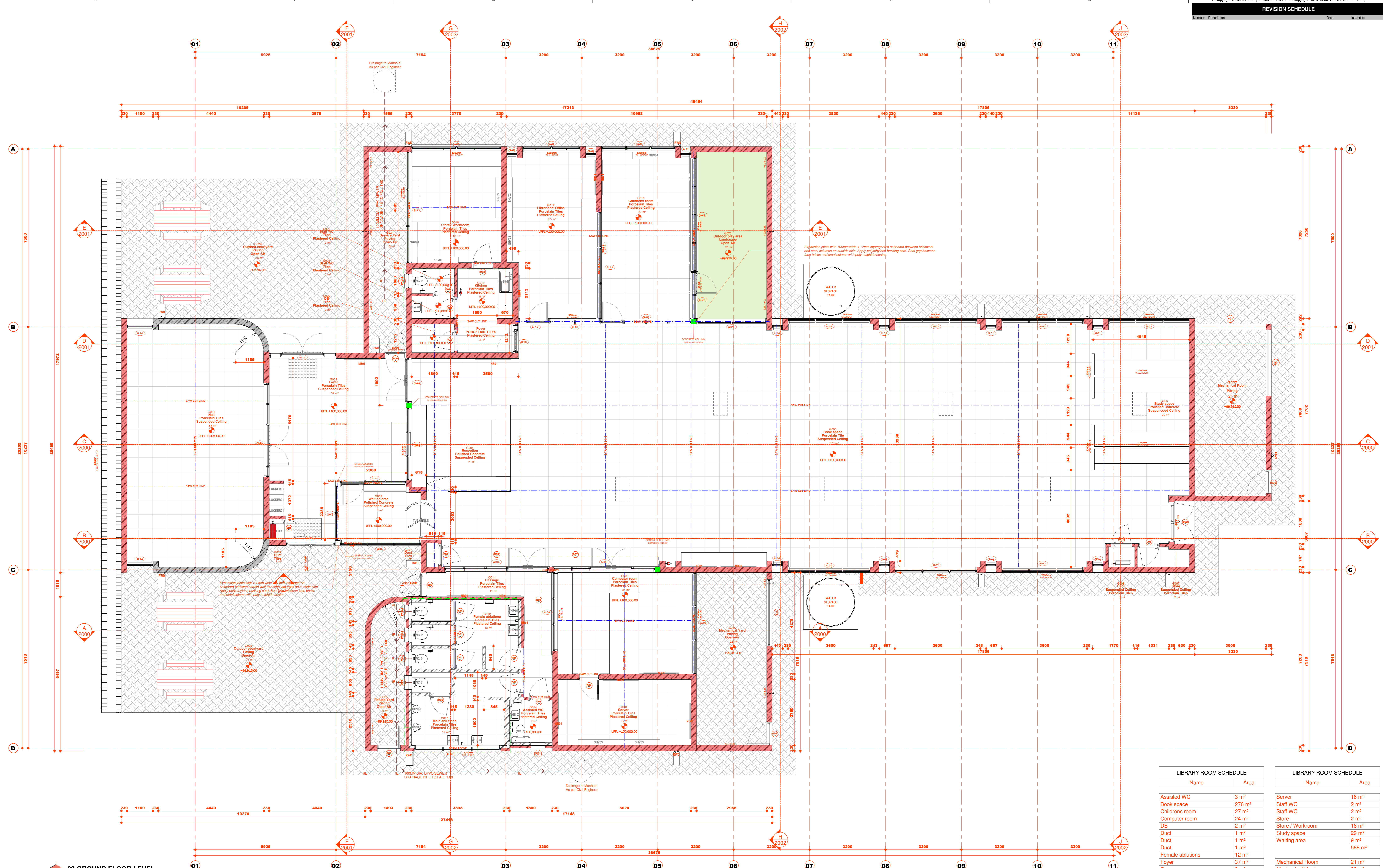
03 GROUND FLOOR LEVEL 1:50
