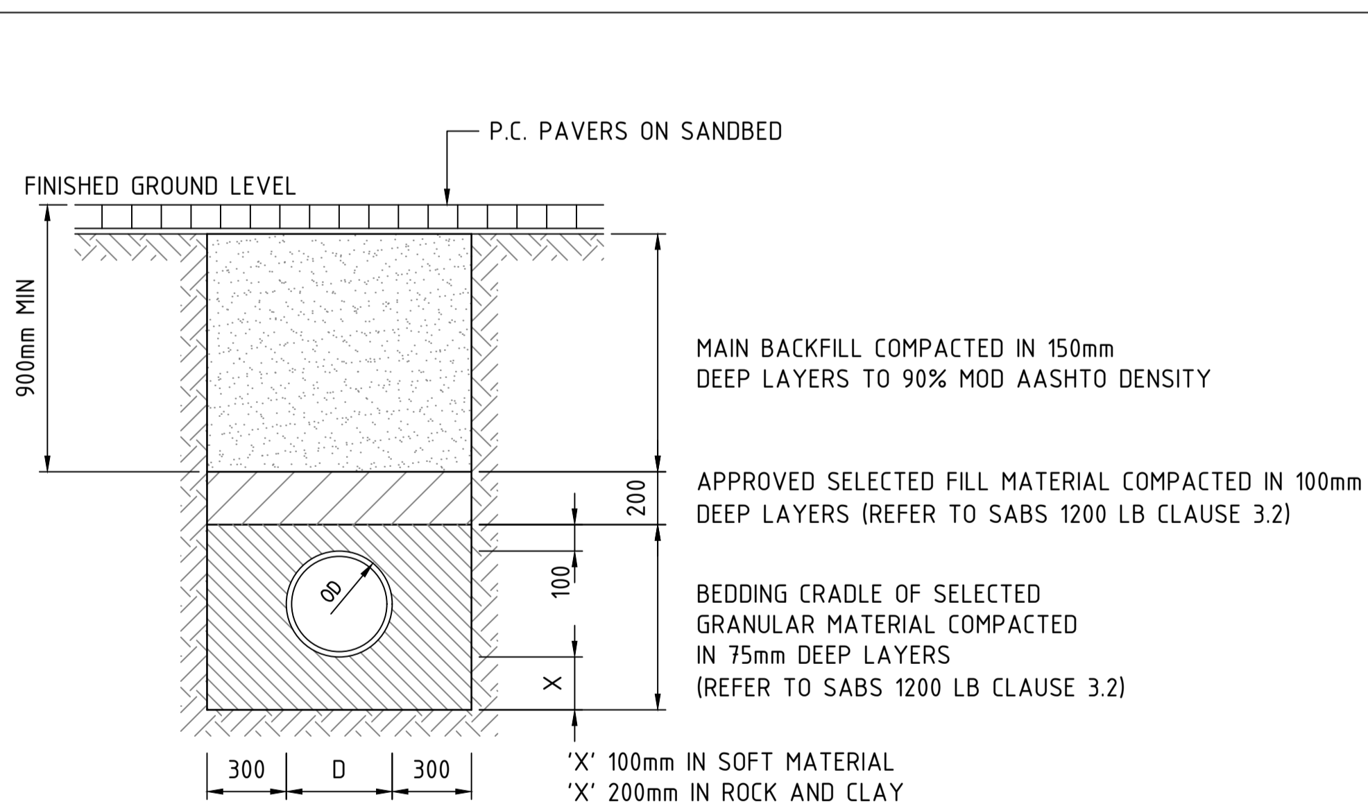
TYPICAL TRENCH SECTION ACROSS PAVED AREAS AND OPEN GROUND SCALE n.t.s
