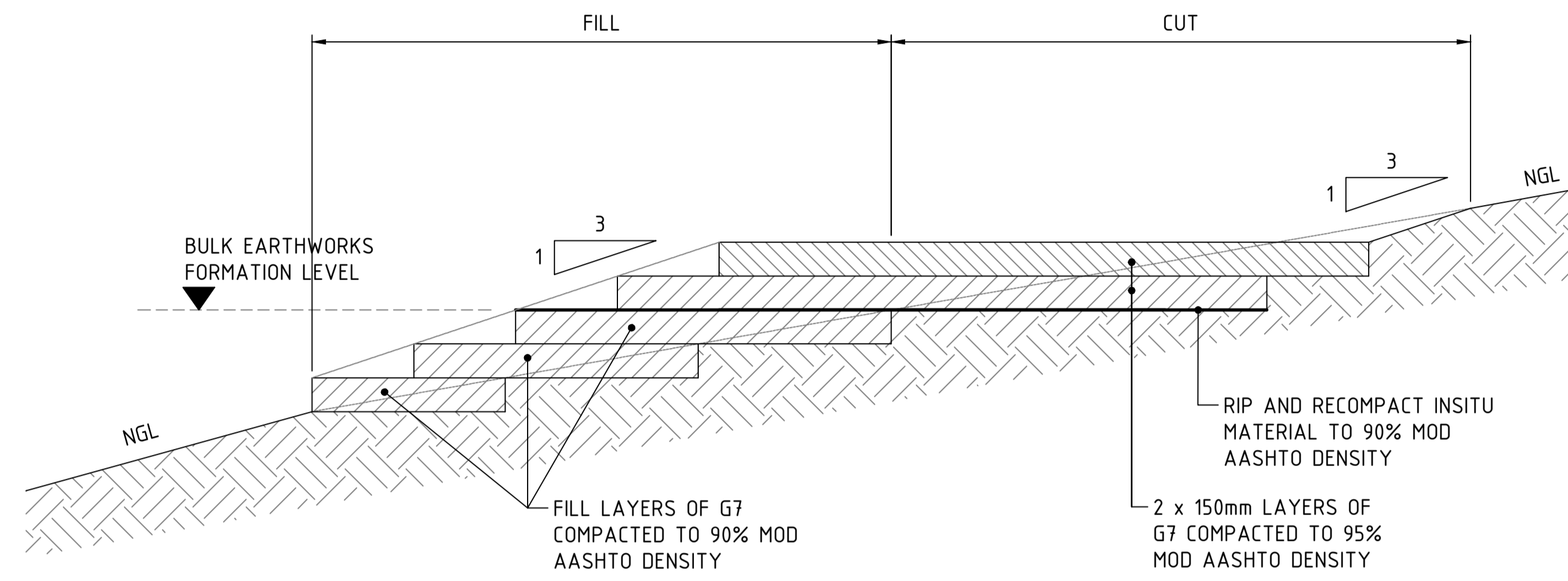
TYPICAL BULK EARTHWORKS SECTION FOR BUILDINGS SCALE 1:20
